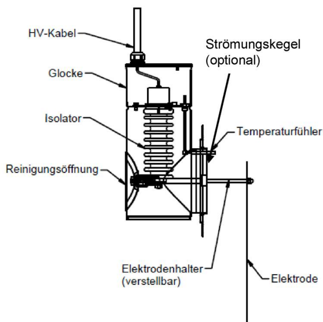
Isolator lang
