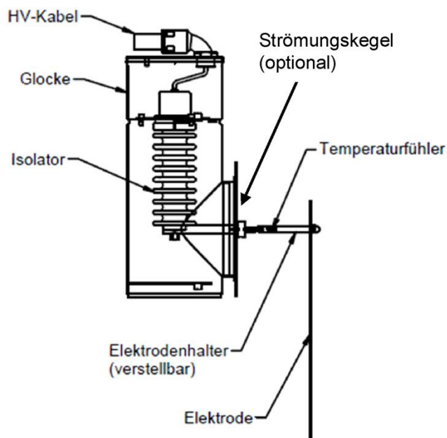
Isolator lang
