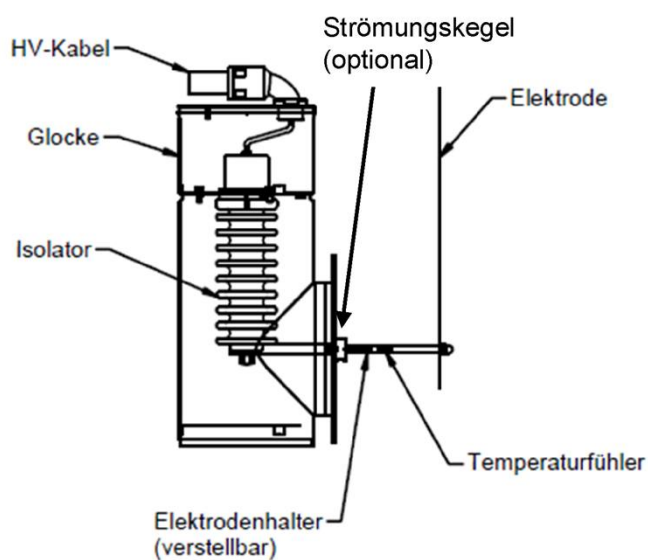
Isolator lang
